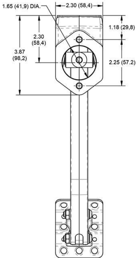
FOOT PAD DETAIL
