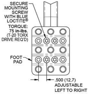
FOOT PAD DETAIL
